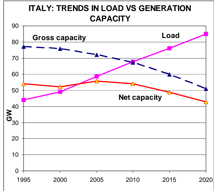
Figure 6.1b: Current and future trend of generation capacity and load in Italy
