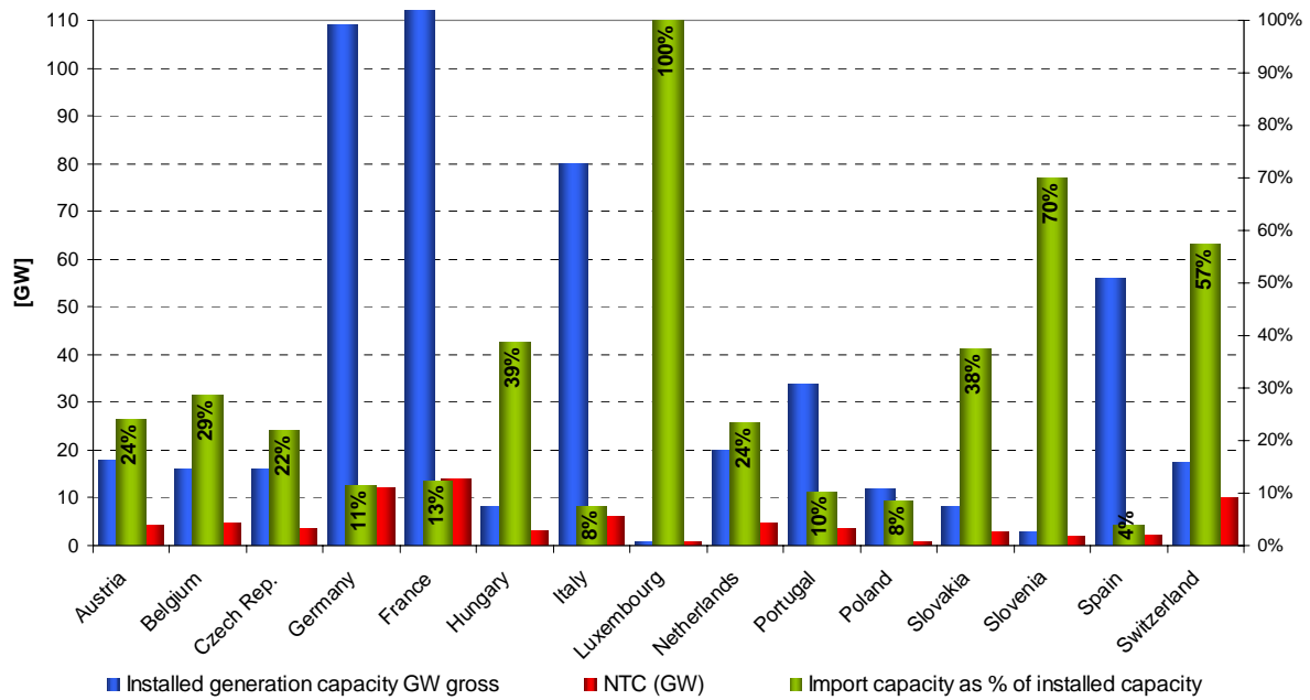
Fig. 5.14 Fig. 5.14 shows installed gross generation capacity, NTC for transmission and import capacity as percentage of installed generation capacity in CE countries. It clearly shows that the import capacity as percentage of installed generation capacity is highest in the smaller countries. This figure also reveals the strategic relevance of Switzerland as a transit country. In absolute terms Switzerland has the highest NTC aside from the largest countries Germany and France. 12
