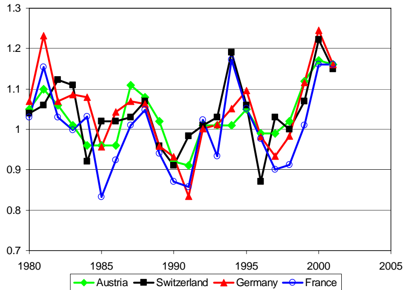
Figure 5.13: Annual variation of Hydro Power availability in CE countries (Source: UCTE and own Investigations)
